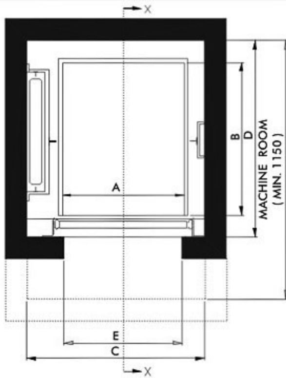
LIFT SHAFT, CAR, C.W. & MACHINE ROOM PLAN
