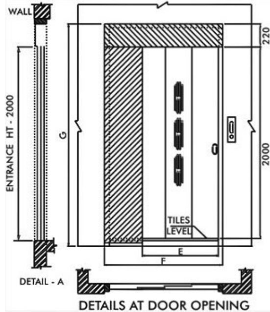
LIFT SHAFT, CAR, C.W. & MACHINE ROOM PLAN
