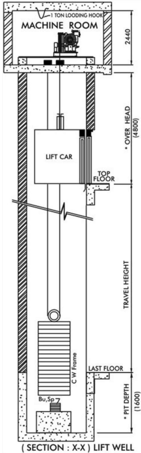
Lift well section
