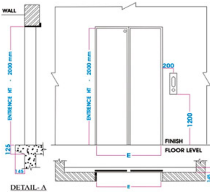
DETAILS AT DOOR OPENING
