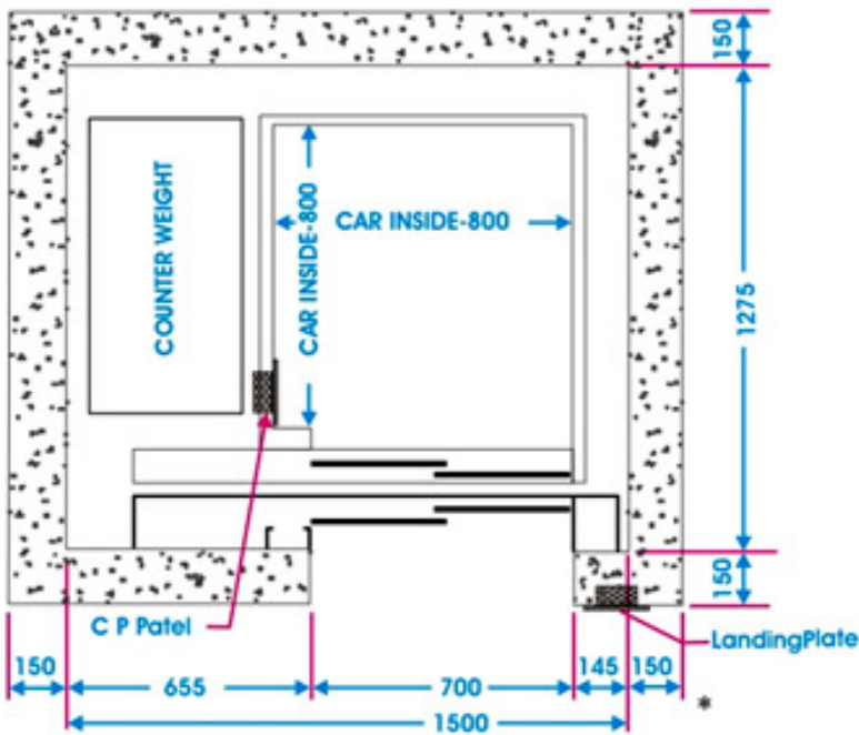
LIFT SHAFT, CAR & C.W. PLAN
